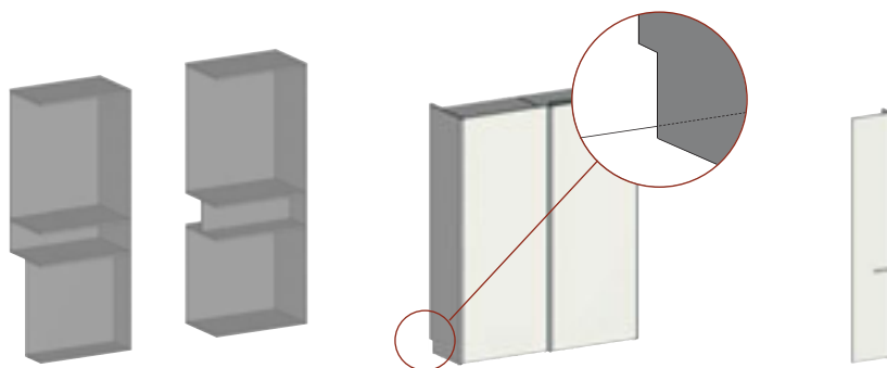
Vano con schienale removibile Compartment with removable back
